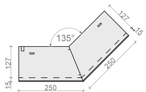
NAROŻNIK ZEWN. 135° ND51/10ALz135°ep, ND51/10Sz135°ep
