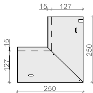
NAROŻNIK WEWN. 90° ND51/10ALwep, ND51/10Swep
