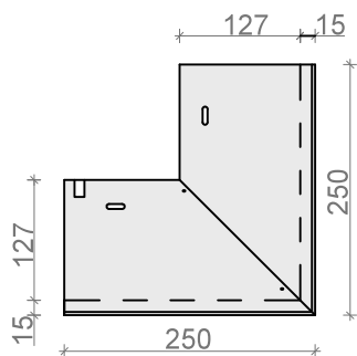
NAROŻNIK ZEWN. 90° ND51/10ALzep, ND51/10Szep
