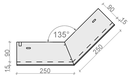
NAROŻNIK ZEWN. 135° ND95/37ALz135°, ND95/37Sz135°
