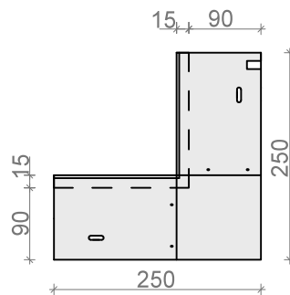
NAROŻNIK WEWN. 90° ND95/37ALw, ND95/37Sw
