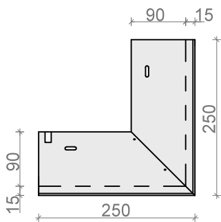
NAROŻNIK ZEWN. 90° ND95/37ALz, ND95/37Sz
