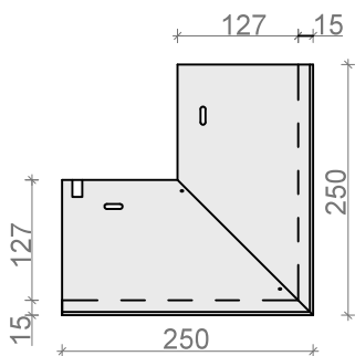
NAROŻNIK ZEWN. 90° ND51/70ALzep, ND51/70Szep
