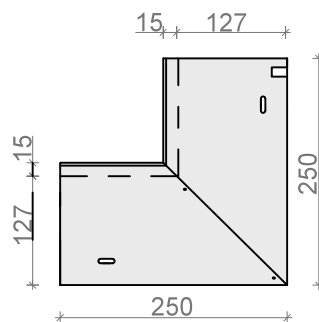
NAROŻNIK WEWN. 90° ND51/70ALwep, ND51/70Swep
