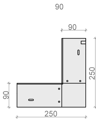
NAROŻNIK WEWN. 90° NKP 10ALw, NKP 10Sw
