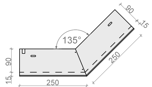
NAROŻNIK ZEWN. 135° ND51/70ALz135°, ND51/70Sz135°
