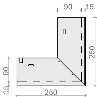
NAROŻNIK ZEWN. 90° ND51/70ALz, ND51/70Sz
