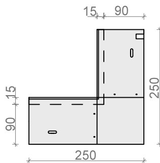
NAROŻNIK WEWN. 90° ND51/70ALw, ND51/70Sw
