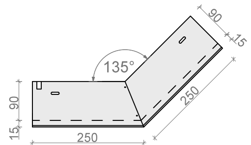
NAROŻNIK ZEWN. 135° ND51/10ALz135°, ND51/10Sz135°
