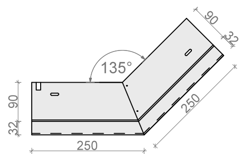
NAROŻNIK ZEWN. 135° ND37/70ALz135°, ND37/70Sz135°
