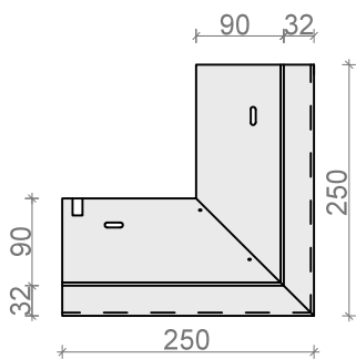
NAROŻNIK ZEWN. 90° ND37/70ALz, ND37/70Sz
