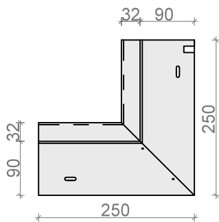
NAROŻNIK WEWN. 90° ND37/70ALw, ND37/70Sw
