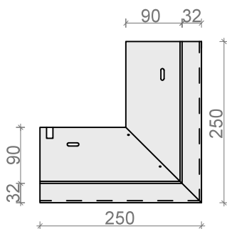
NAROŻNIK ZEWN. 90° ND37/10ALz, ND37/10Sz
