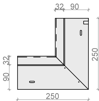
NAROŻNIK WEWN. 90° ND37/10ALw, ND37/10Sw
