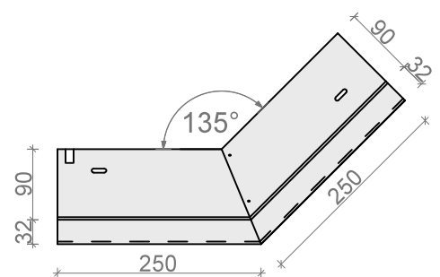
NAROŻNIK ZEWN. 135° ND37/10ALz135°, ND37/10Sz135°
